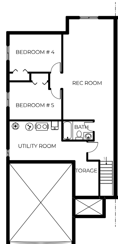
OPTIONAL FINISHED LOWER LEVEL VERSION 'B' 770 SQ.FT.
