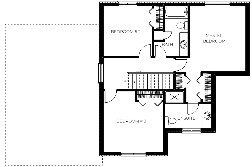
SECOND FLOOR PLAN 840 SQ.FT. SECOND FLOOR AREA
