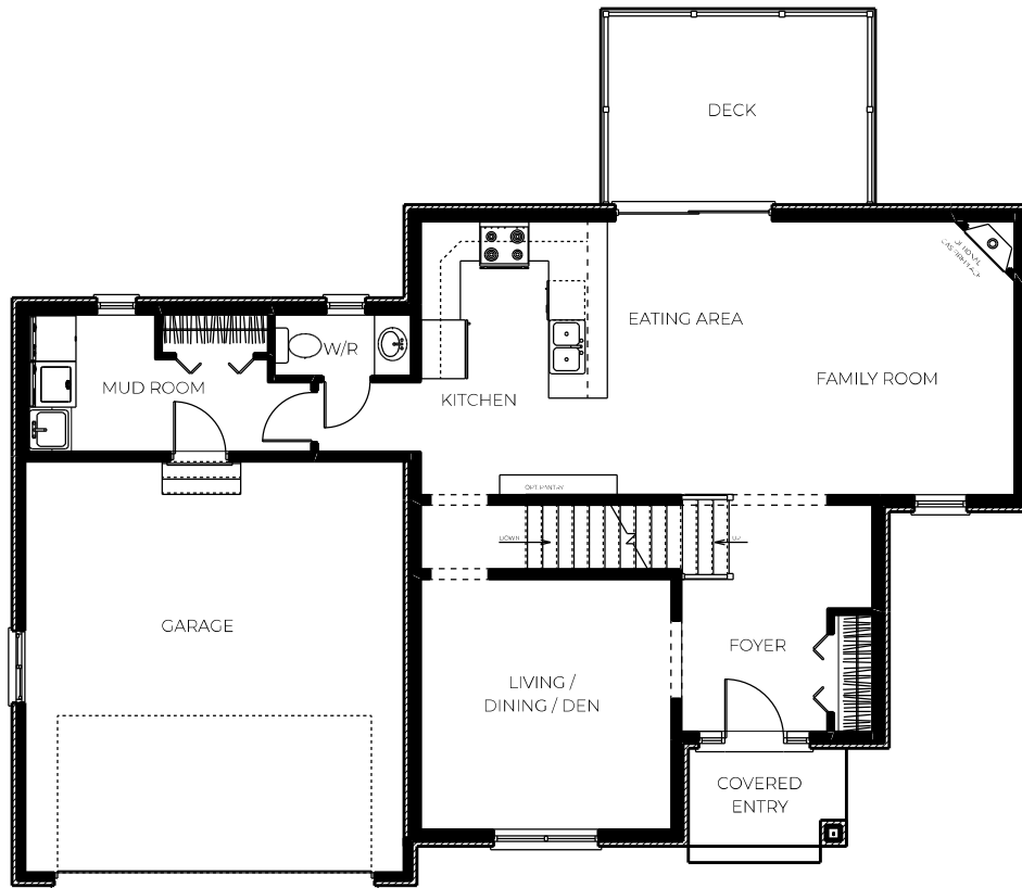
MAIN FLOOR PLAN 1,040 SQ.FT. MAIN FLOOR AREA
