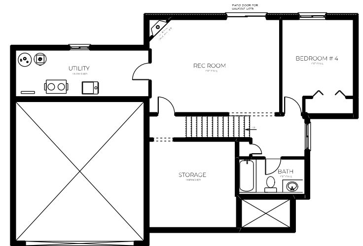
BASEMENT PLAN
