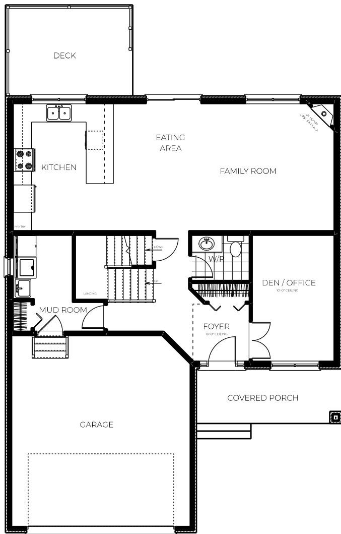
MAIN FLOOR PLAN 1,040 SQ.FT. MAIN FLOOR AREA
