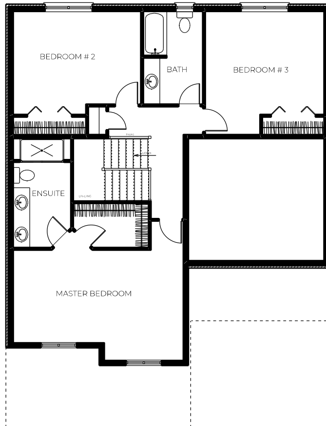
SECOND FLOOR PLAN 1,020 SQ.FT. SECOND FLOOR AREA
