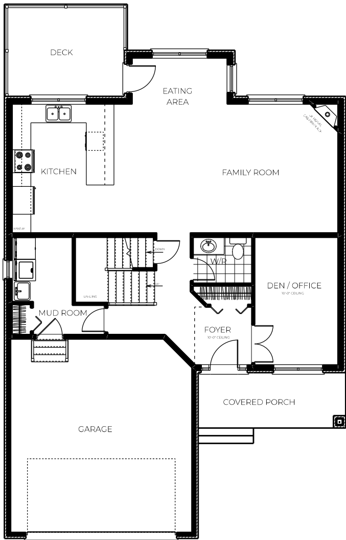
MAIN FLOOR PLAN 1,100 SQ.FT. MAIN FLOOR AREA
