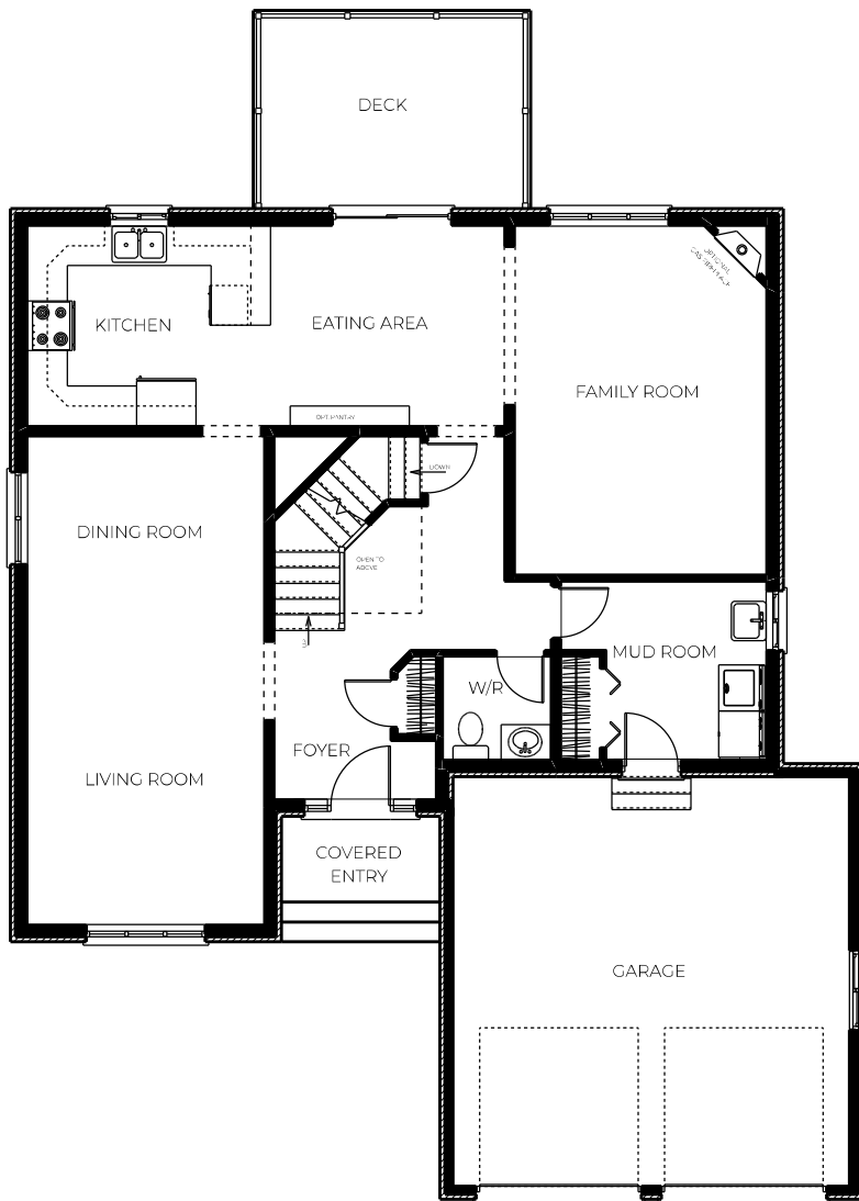
MAIN FLOOR PLAN 1,250 SQ.FT. MAIN FLOOR AREA
