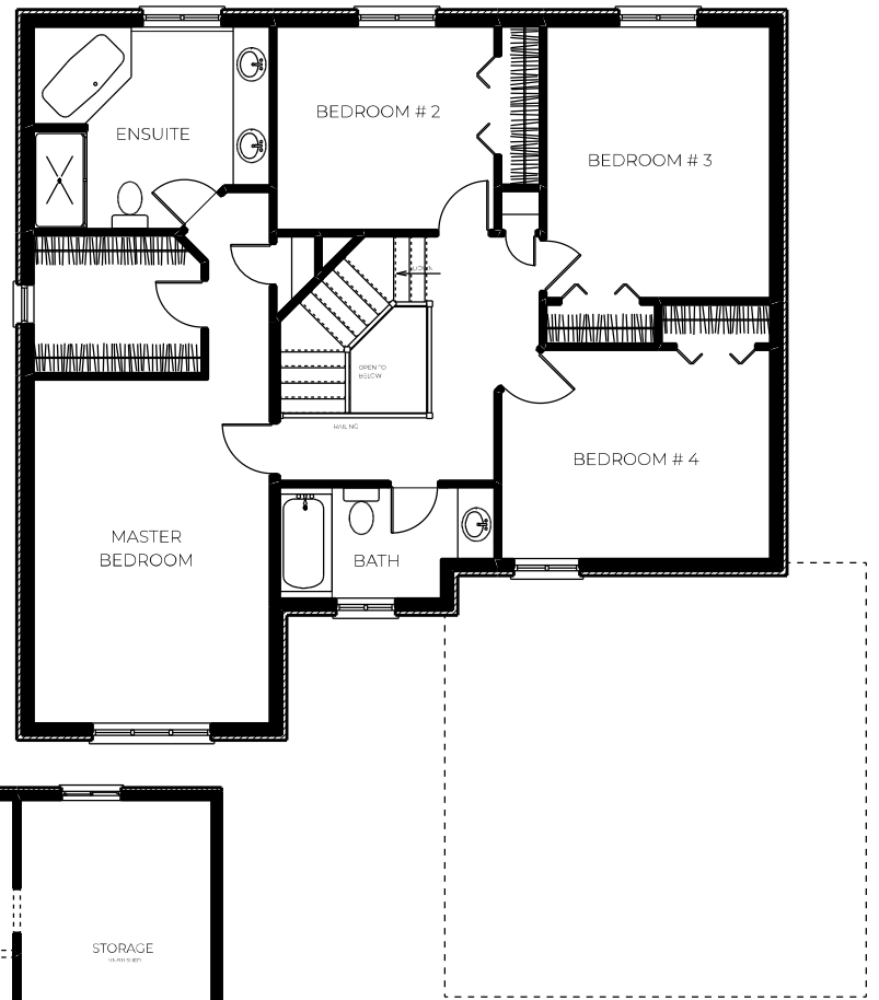
SECOND FLOOR PLAN 1,190 SQ.FT. SECOND FLOOR AREA
