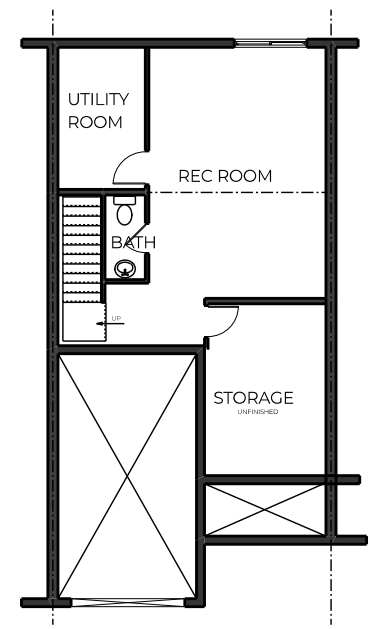
OPTIONAL FINISHED LOWER LEVEL 365 SQ.FT.
